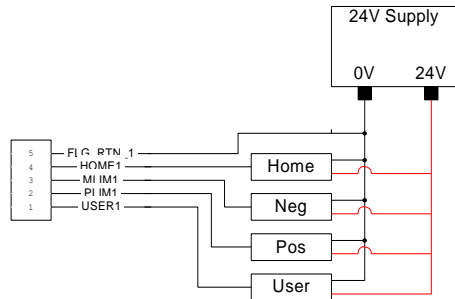
ACC-24E2 Sourcing Flags
