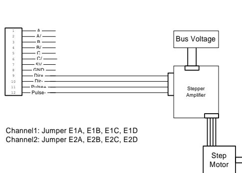
ACC-24E2 PFM-Stepper Output
