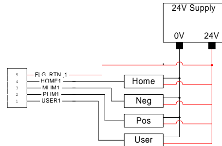
ACC-24E2 Sinking Flags
